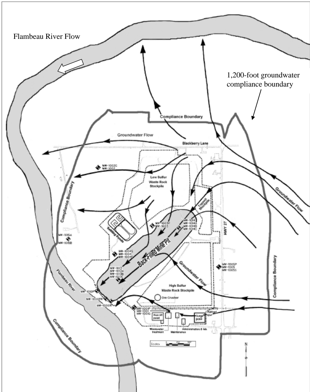
Figure A: Plan View Groundwater Flow
